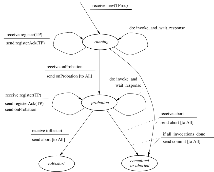
Figure 5: Finite state automaton of a transaction manager
