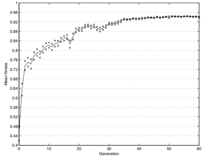
Figure 3: Mean fitness of the GA population with one standard error
