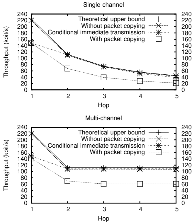
Figure 5: Multi-hop raw bit throughput with conditional immediate transmission is 97% of the theoretical upper bound on 802.15.4 throughput. This does not take packet headers into account; an 8 byte packet header limits the application data throughput to 104 kbit/s for the 6-hop multi-channel case.
