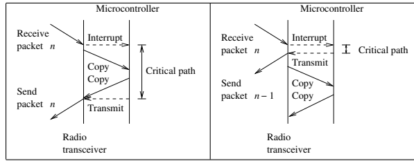
Figure 1: Packet forwarding with packet copying (left) and packet forwarding with conditional immediate transmission (right). With conditional immediate transmission, packet copying is done after forwarding the packet.
