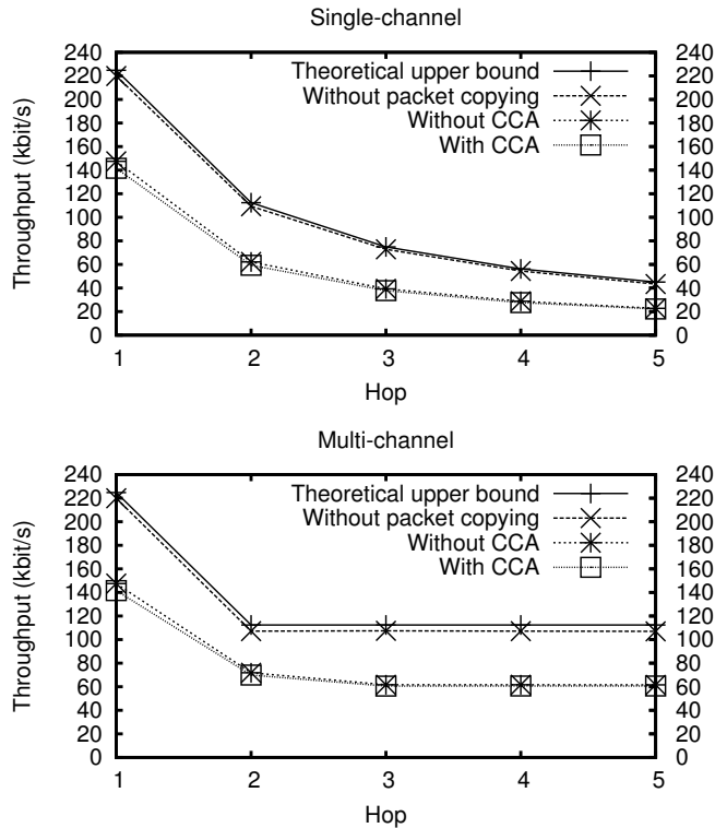
Figure 4: Experimental results of multi-hop 802.15.4 throughput with a single channel (top) and multiple channels (bottom). Packet copying nearly halves the throughput both in the single-channel case and in the multi-channel case. Clear-channel assessment (CCA) has little impact on throughput.
