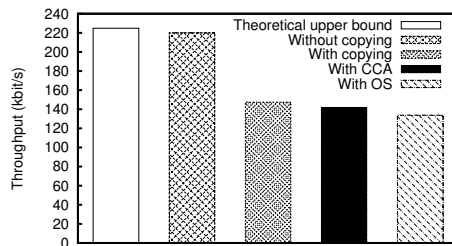
Figure 3: Packet copying reduces the single-hop throughput with one third: from 220 kbit/s to 148 kbit/s. The impact of clear-channel assessment (CCA) and the operating system (OS) is smaller.
