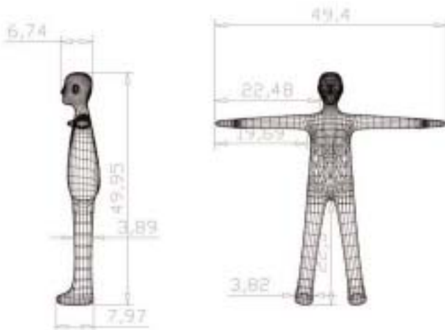
Figure 5: Model and dimensions of SenToy
