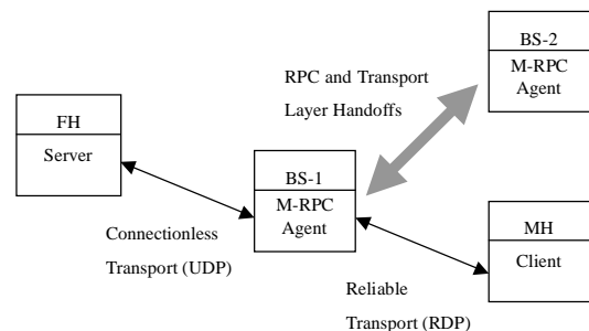
Figure 4. Overview of M-RPC System [1]
