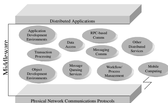
Figure 1. Middleware Segmentation [4]
