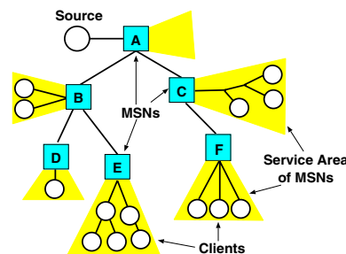
Fig. 1. OMNI Architecture.
