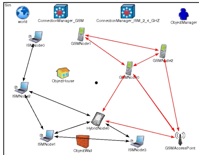
Figure 2: Illustration of a MiXiM Simulation
